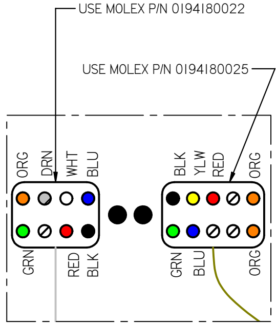
DETAIL A
